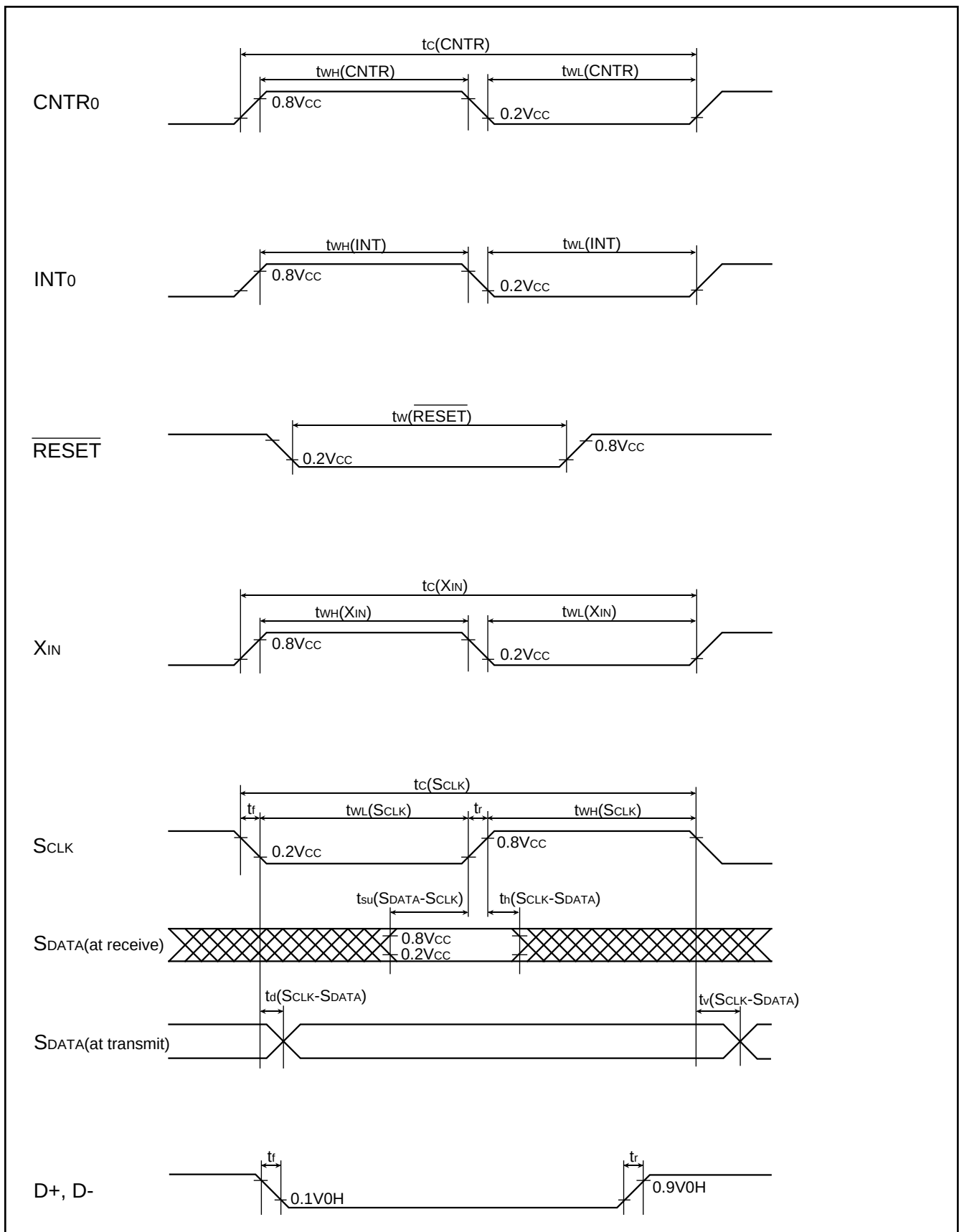
Fig. 49 Timing chart
