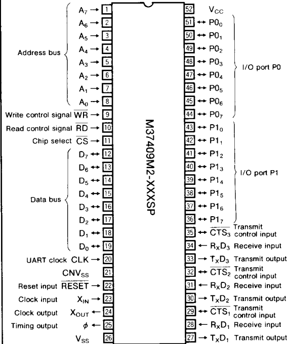
Outline 52P4B
