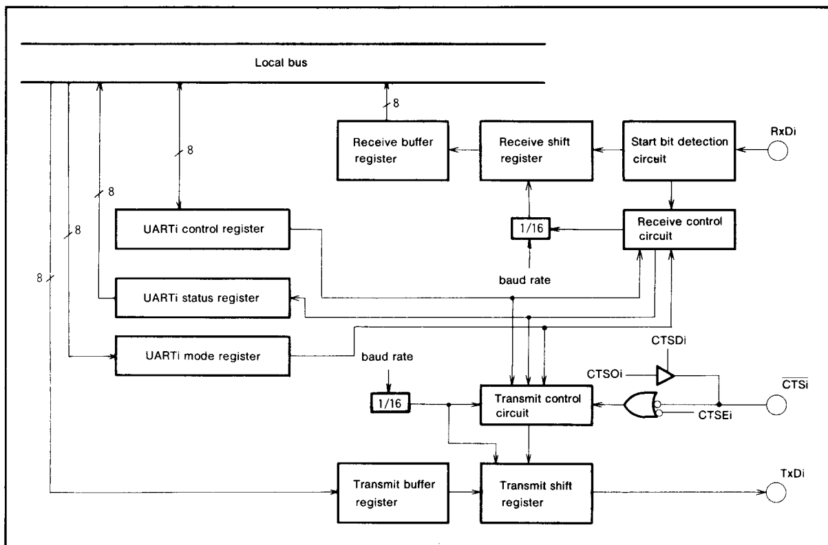
Fig. 10 UARTi block diagram
