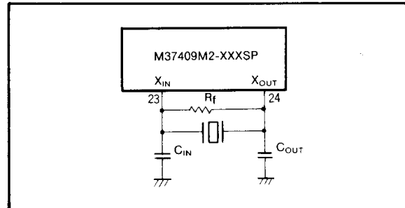
Fig. 19 External ceramic resonator circuit
