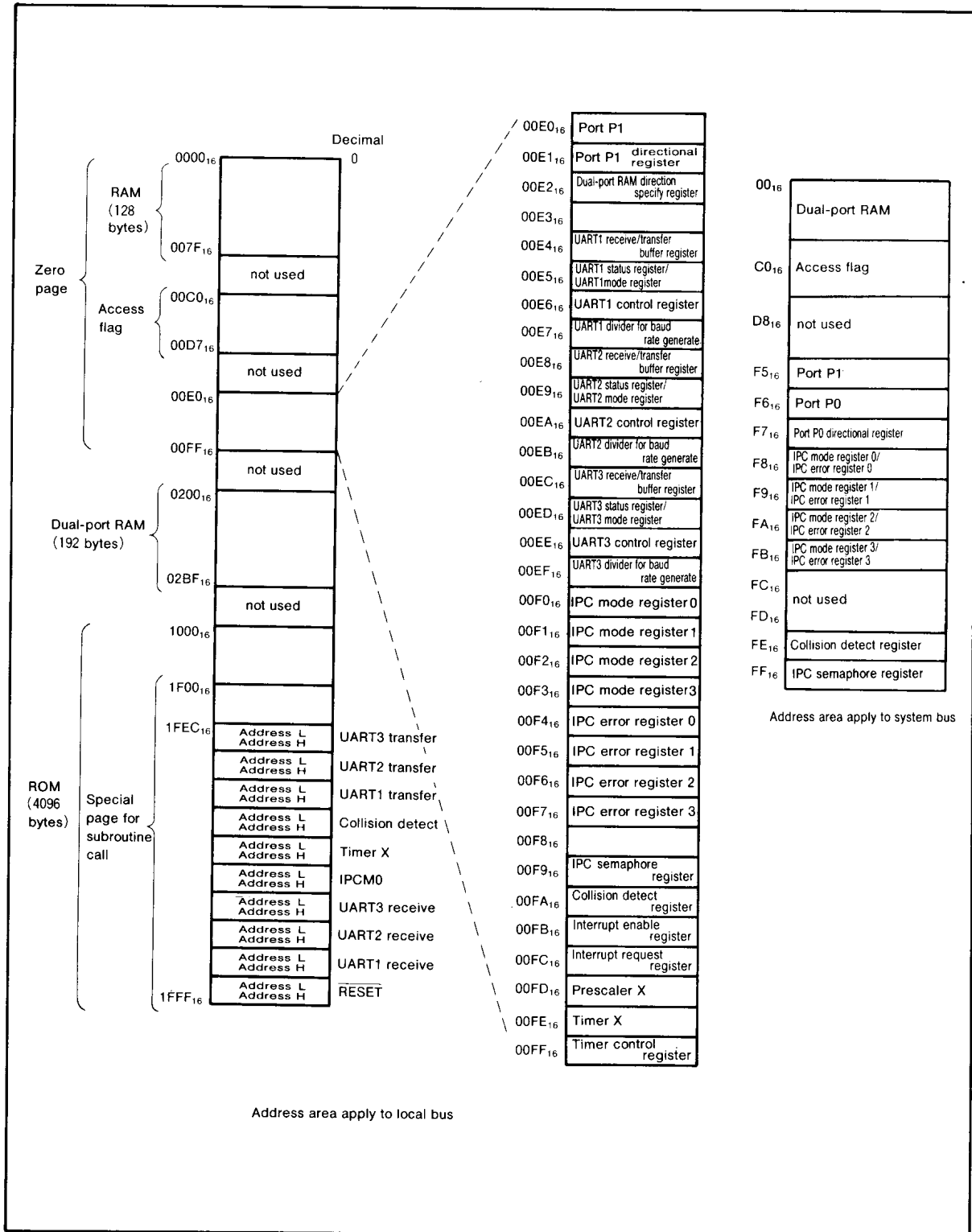
Fig. 1 Memory map
