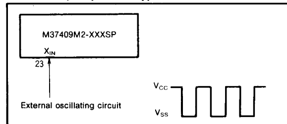
Fig. 21 External clock input circuit
