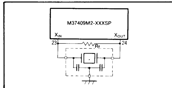
Fig. 20 External ceramic resonator circuit (capacity built-in type)
