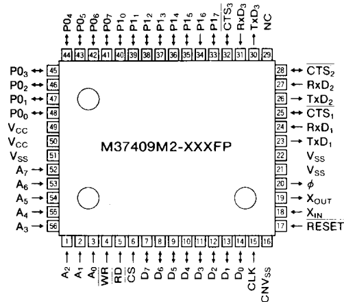
Outline 56P6N
