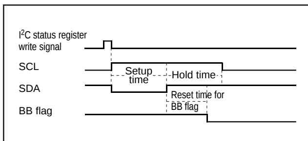
Fig. 12.6.10 STOP Condition Generation Timing Diagram
