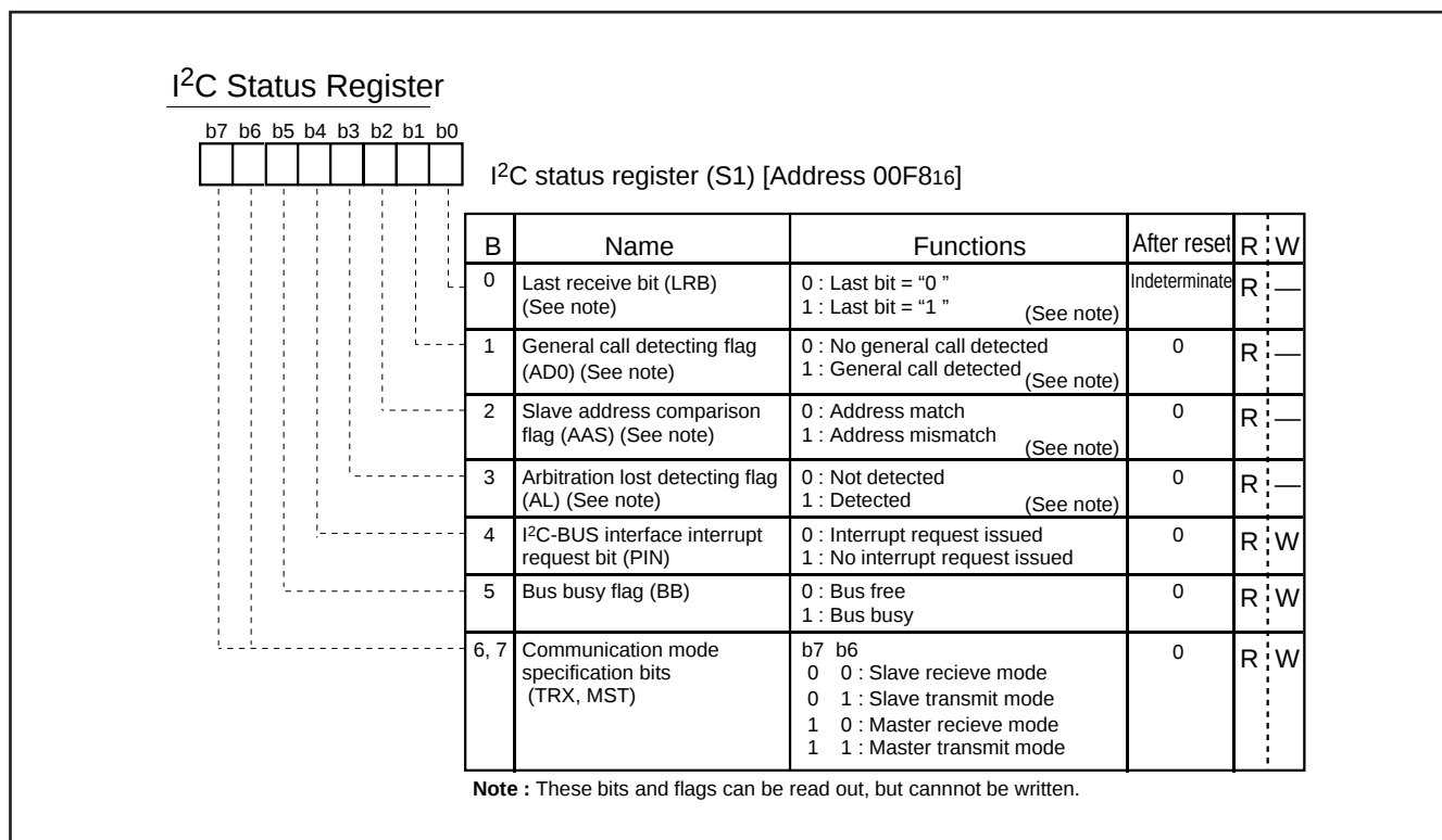
Fig. 12.6.7 I 2 C Status Register
