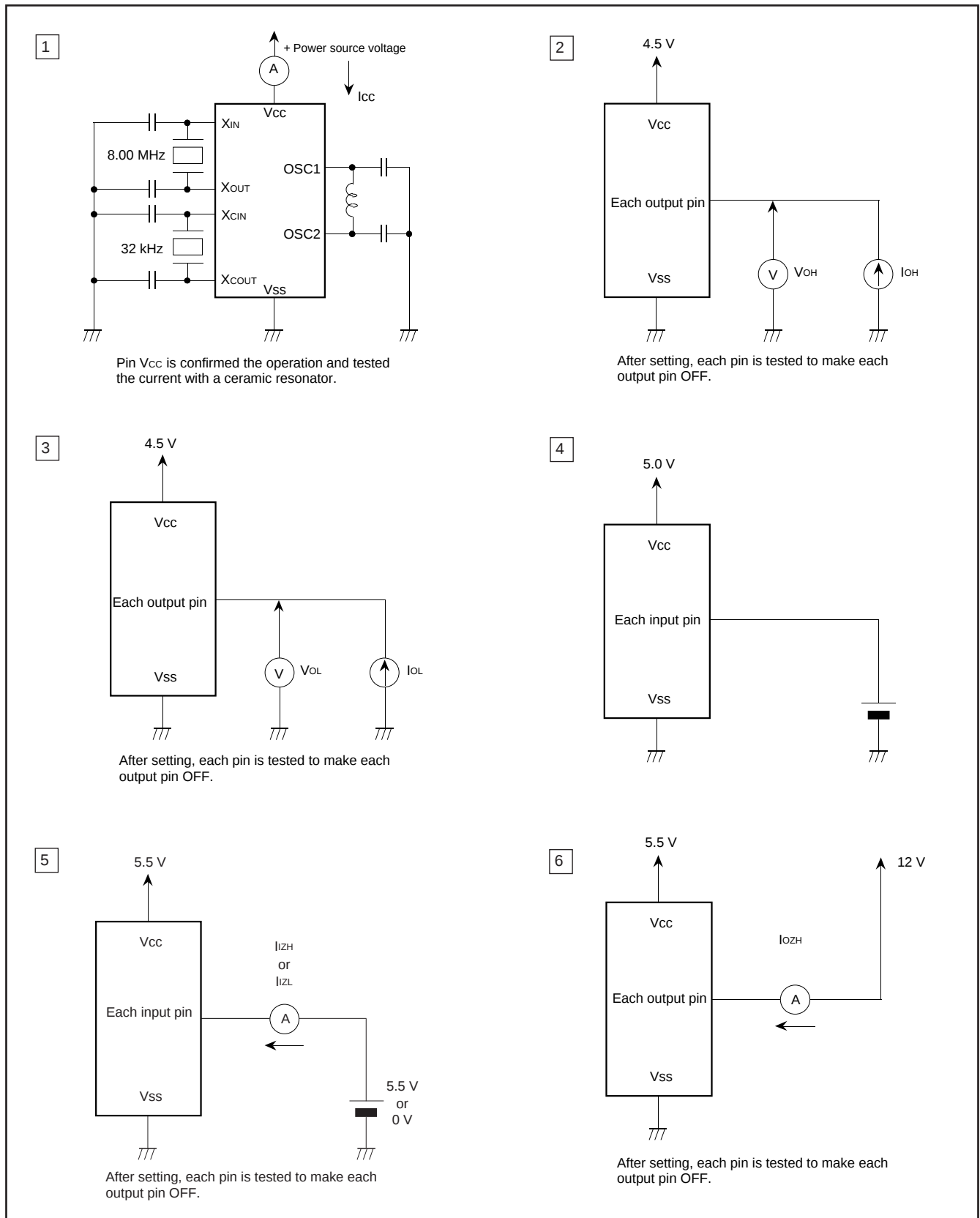
Fig.23.1 Test circuit
