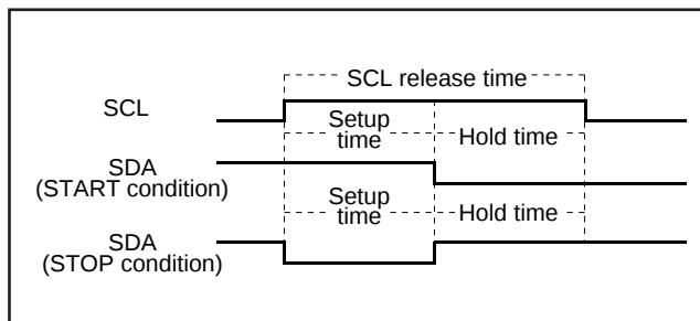
Fig. 12.6.11 START Condition/STOP Condition Detect Timing Diagram
