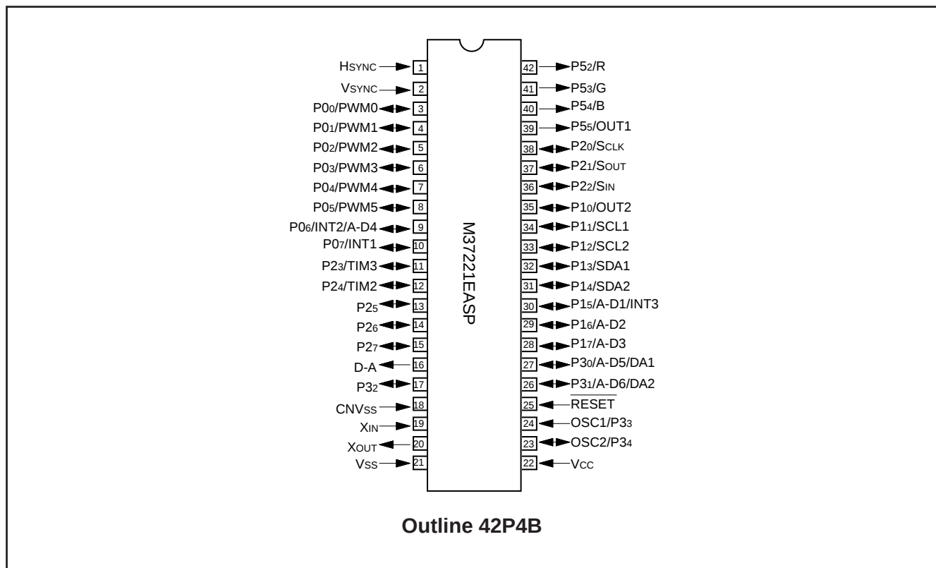
Fig. 4.3 Pin Configuration (3) (Top View)
