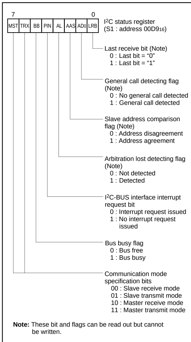
Fig. 17. Structure of I 2 C status register
