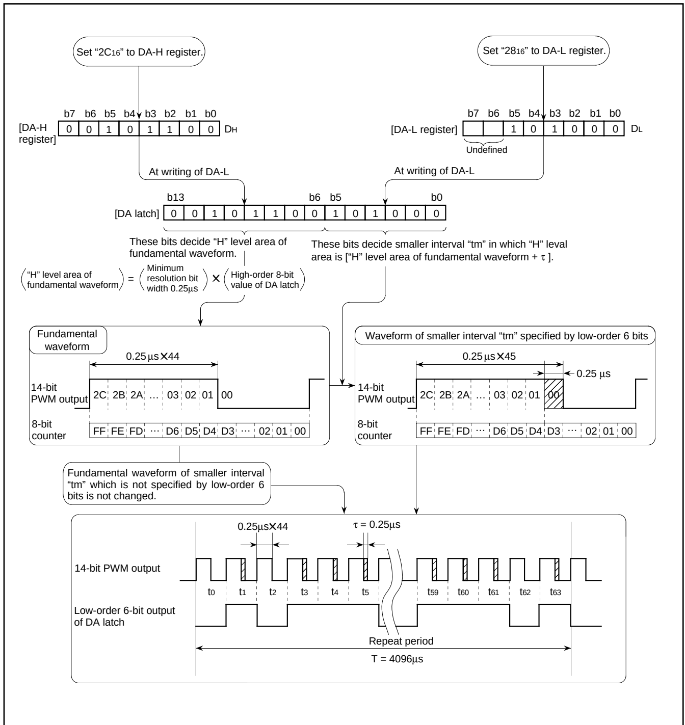
Fig. 25. 14-bit PWM output example ( f(X_{IN}) = 8\text{ MHz} )
