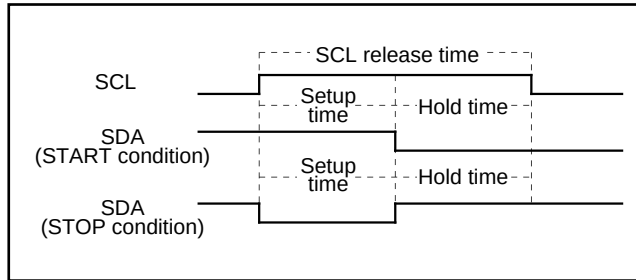
Fig. 21. START condition/STOP condition detecting timing diagram
