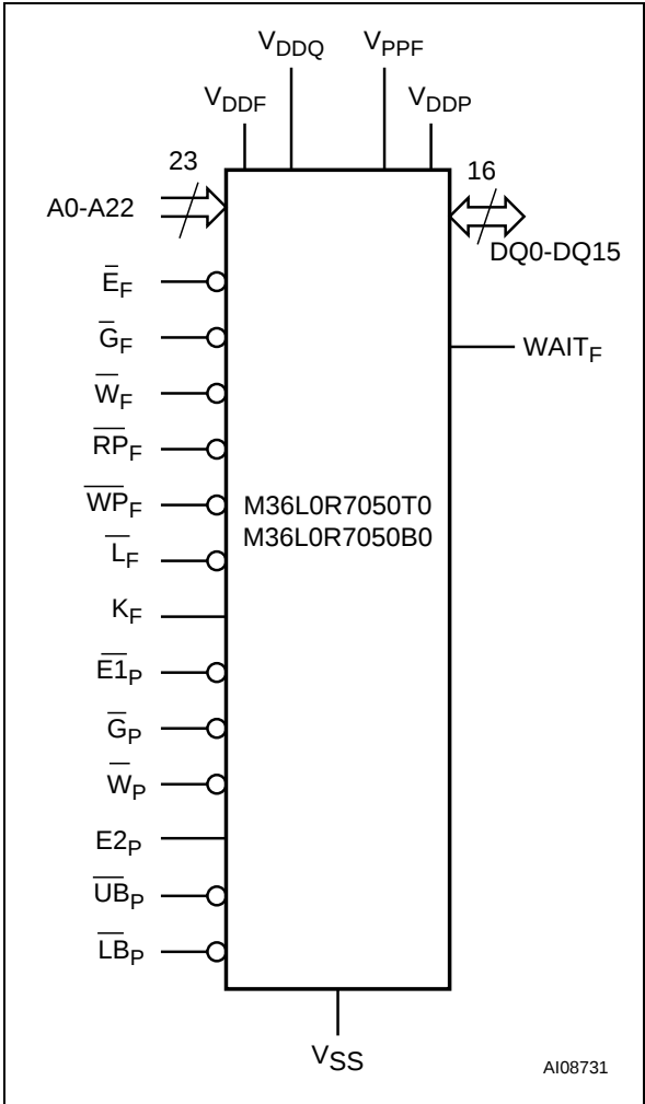
Figure 2. Logic Diagram
