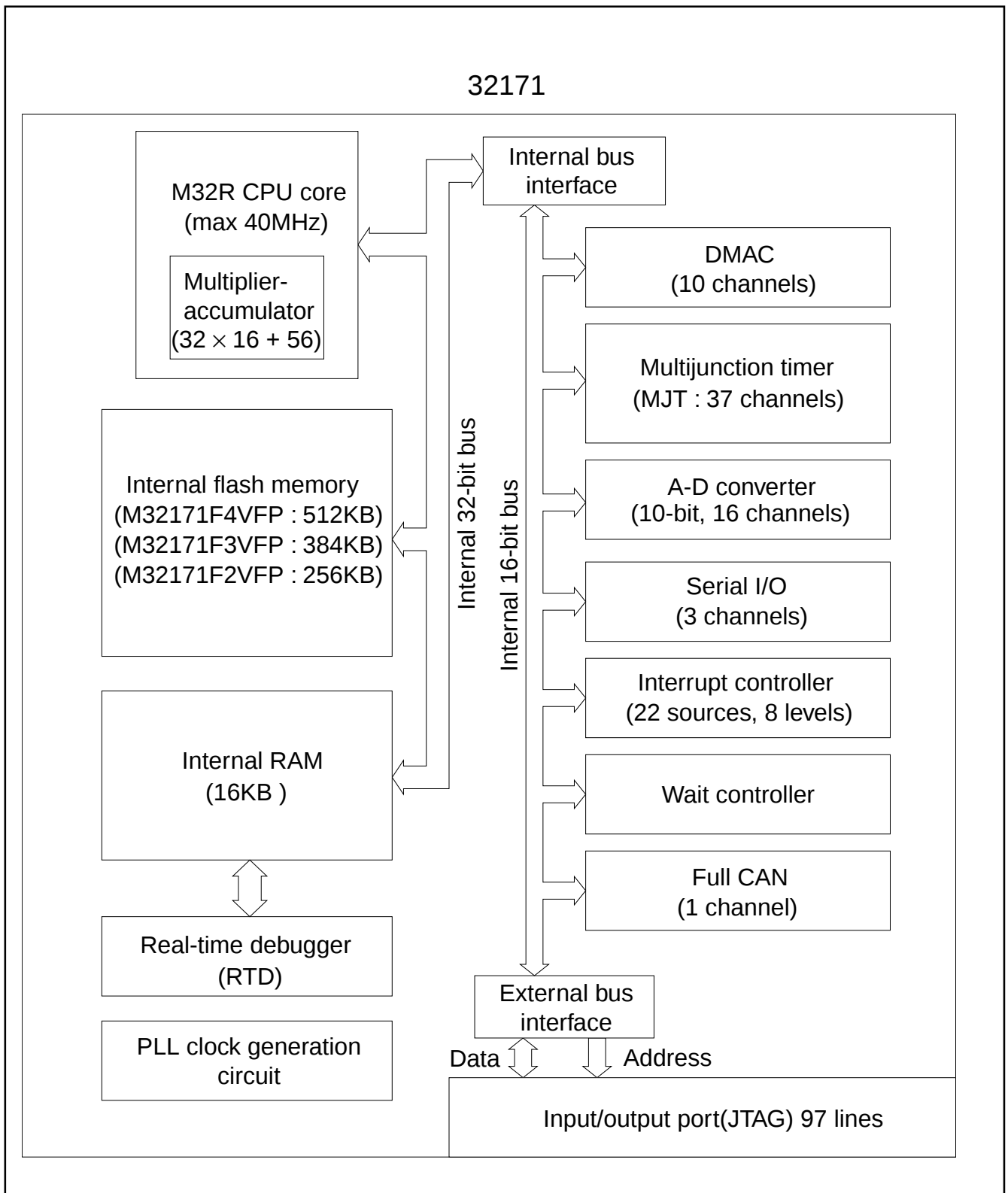
Figure 2 Block diagram
