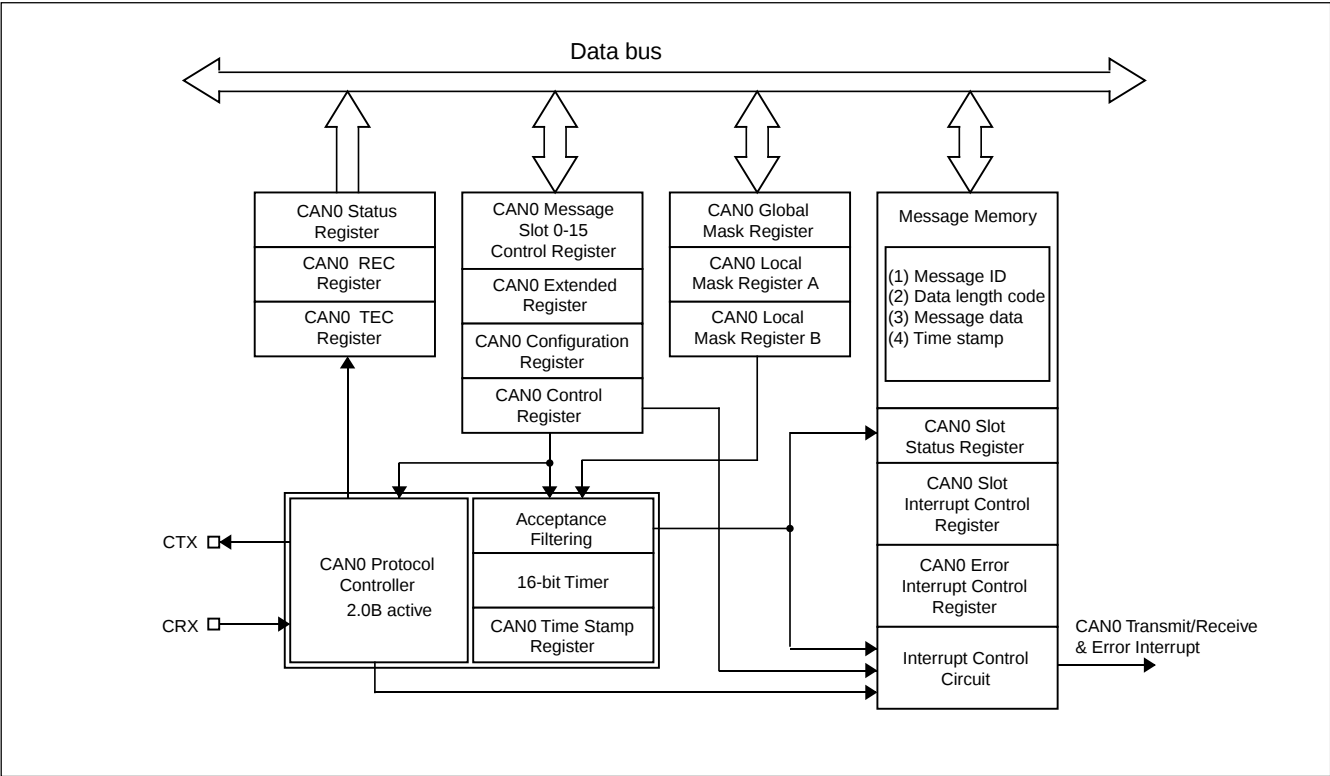
Figure 18 Block Diagram of the CAN Module
