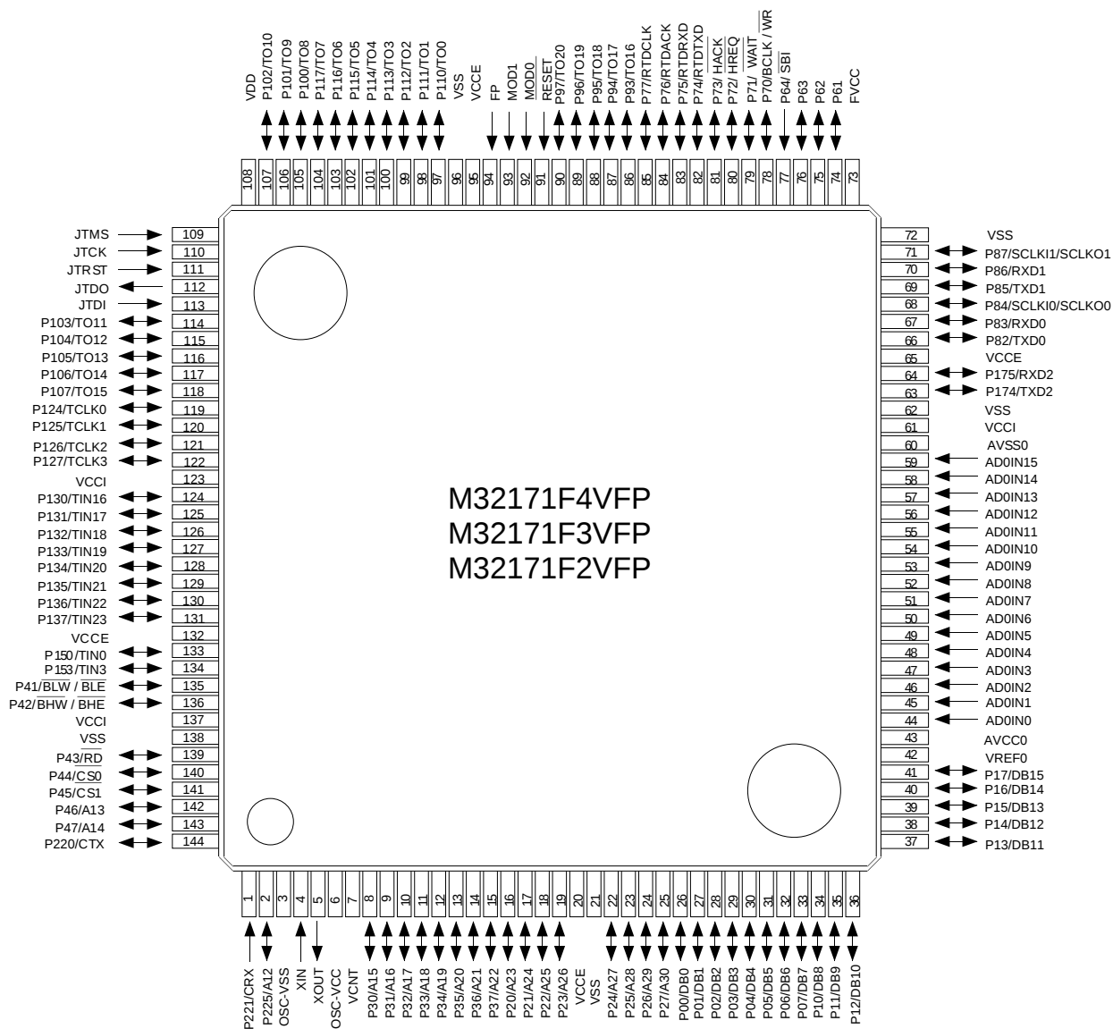
Pin Assignment(top view)
