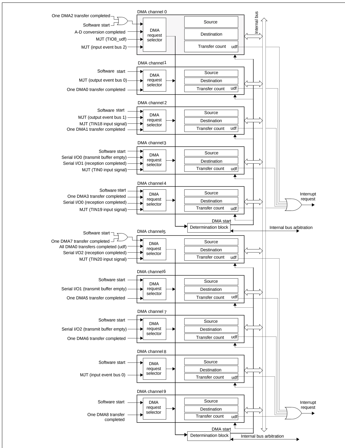
Figure 11 Block Diagram of the DMAC
