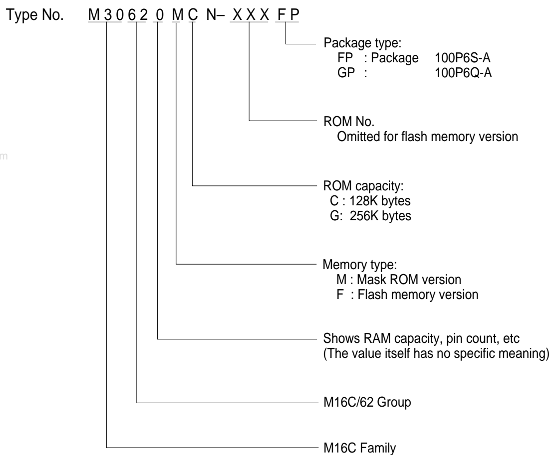
Figure 1.1.5. Type No., memory size, and package
