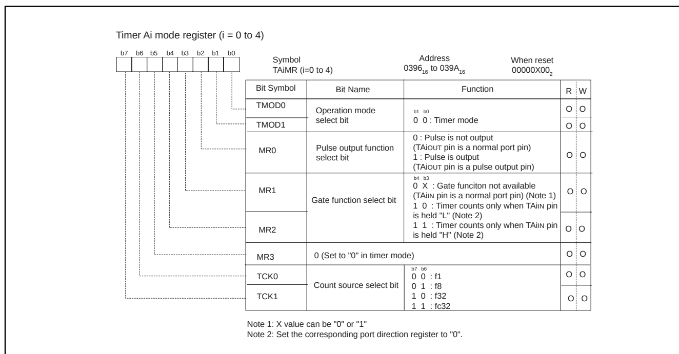
Figure 1.81. Timer Ai mode register in timer mode
