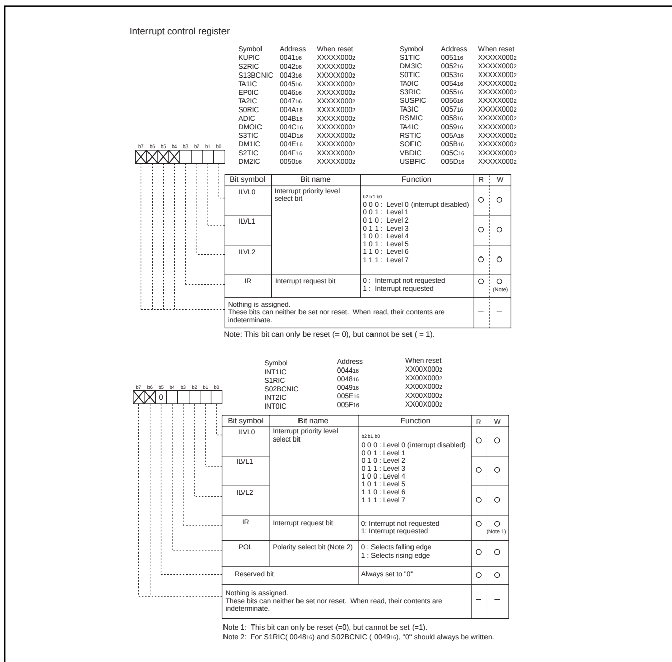
Figure 1.31. Interrupt control registers control registers
