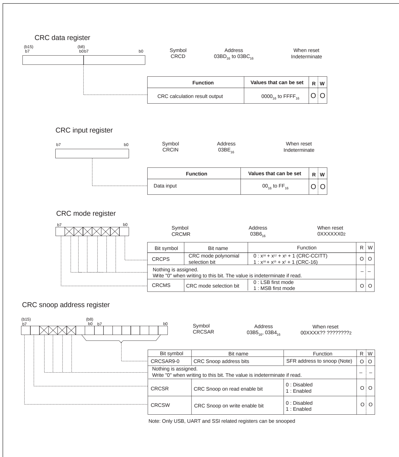
Figure 1.130. CRC-related registers
