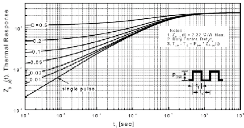
Transient Thermal Response Curve For JCS2N60V/R/S/B/C
