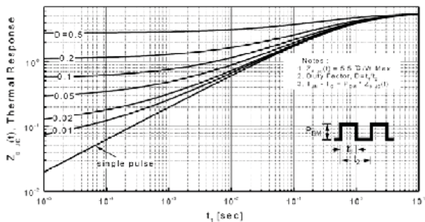
Transient Thermal Response Curve For JCS2N60F
