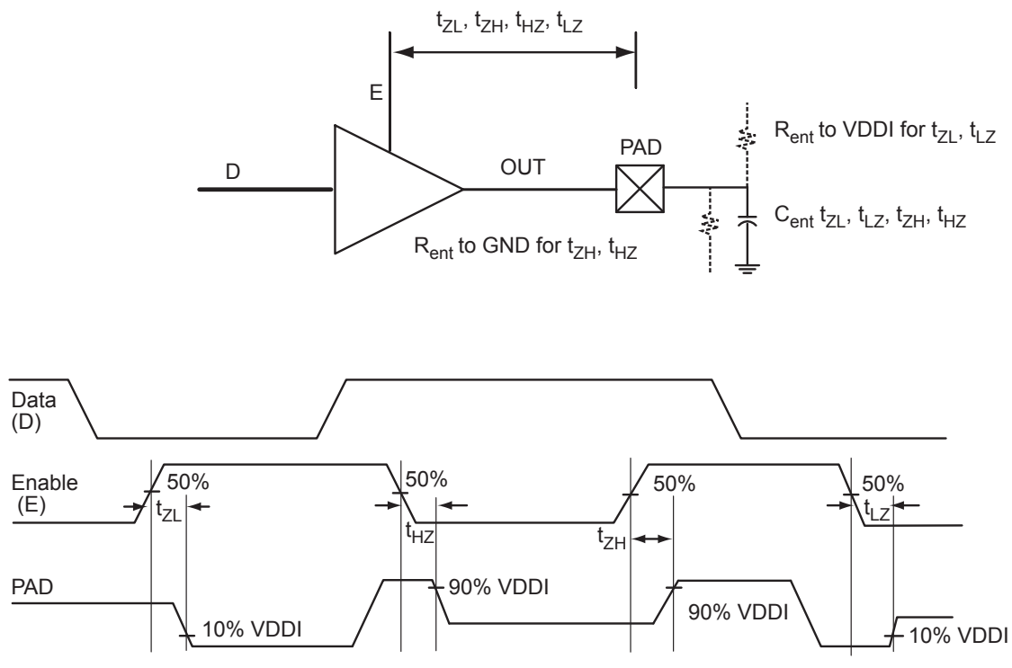
Figure 2 • Tristate Buffer for Enable Path Test Point
