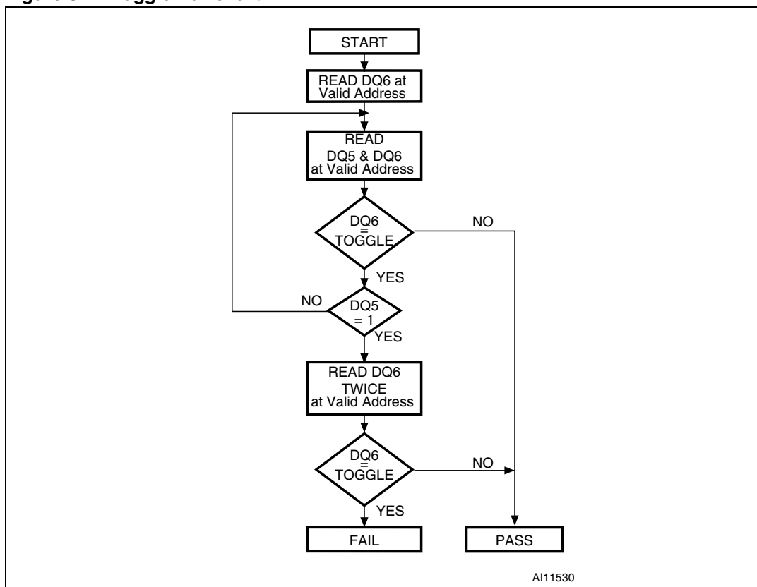
Figure 6. Toggle flowchart
