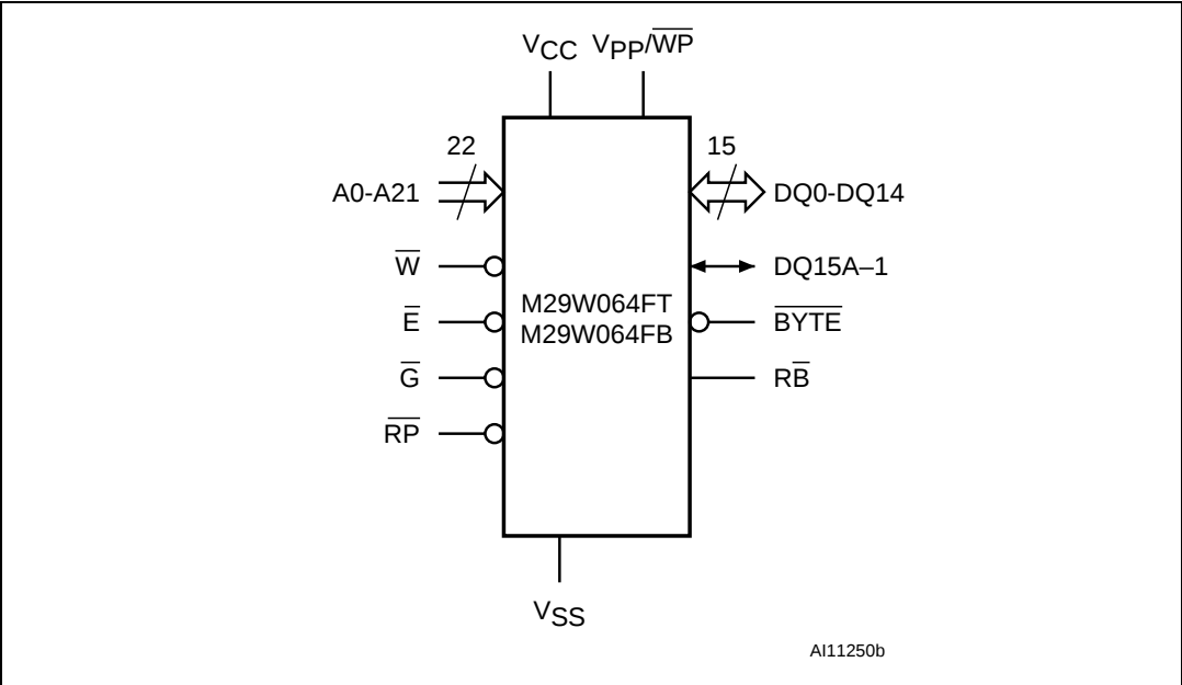
Figure 1. Logic diagram
