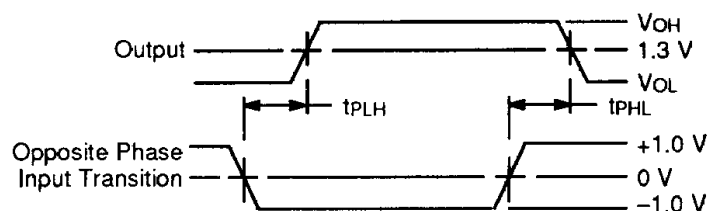
Propagation Delay (Notes 1 and 3)
