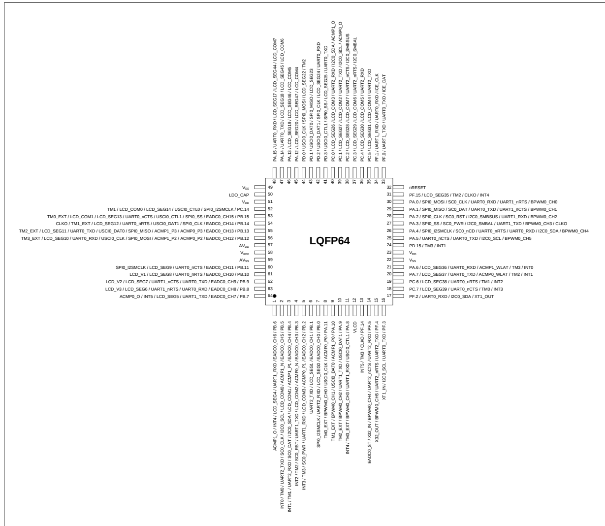
Figure 4.1-6 M254SD2AE Multi-function Pin Diagram
