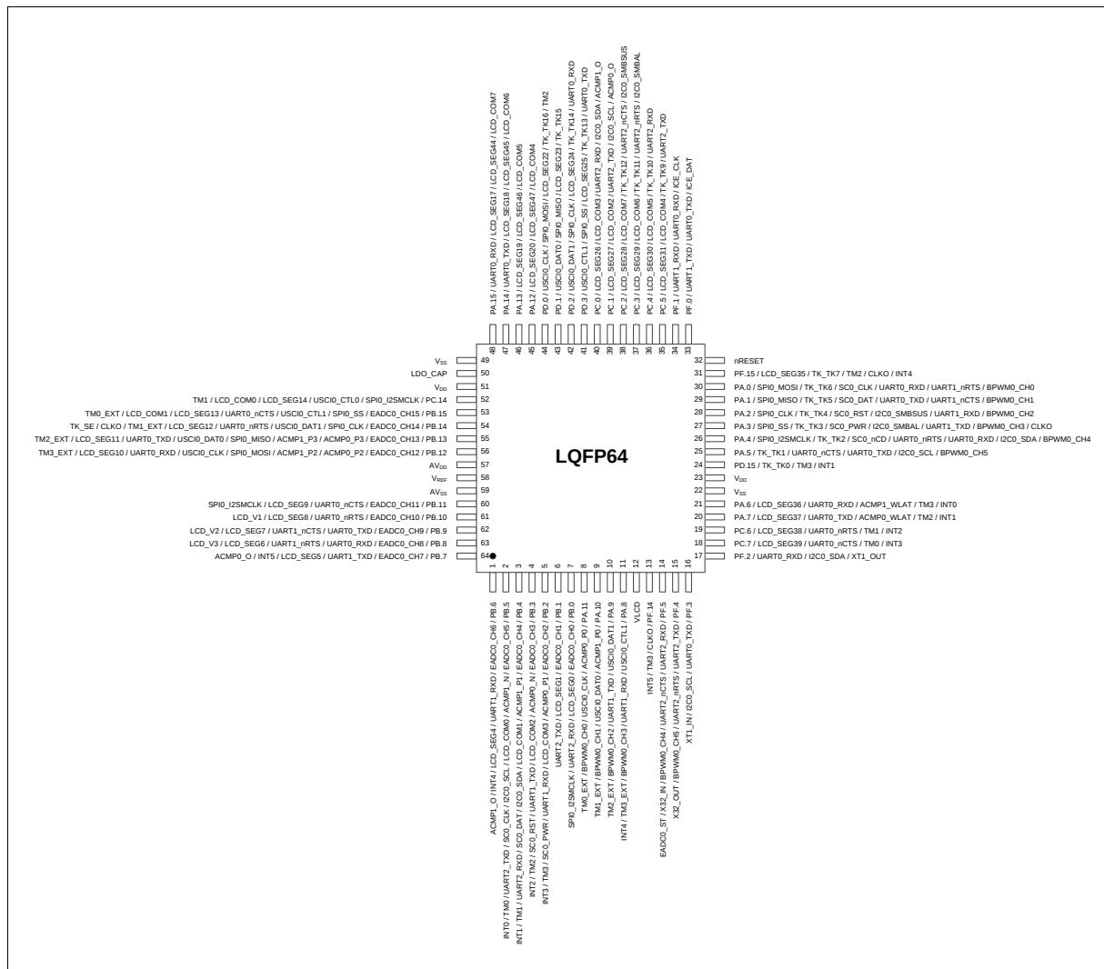
Figure 4.1-16 M256SD2AE Multi-function Pin Diagram
