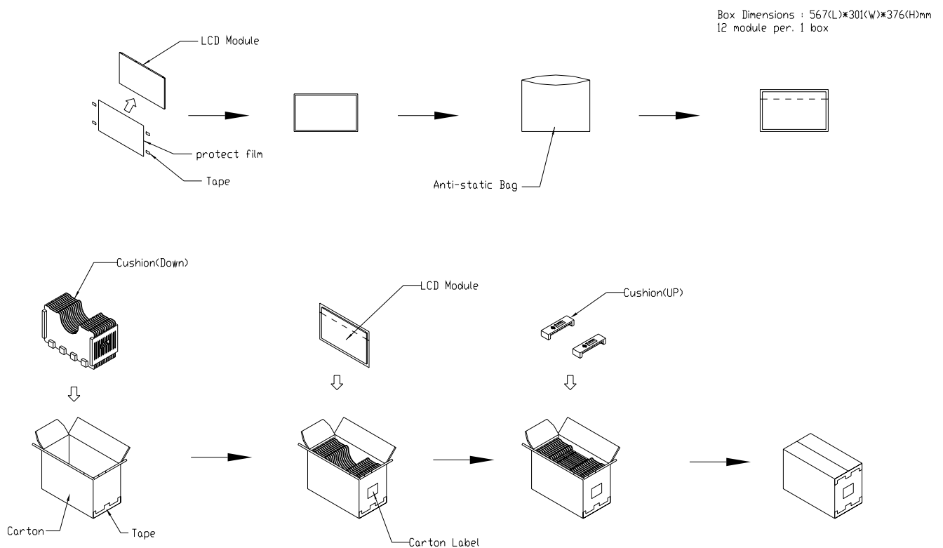
Figure. 7-1 Packing method
