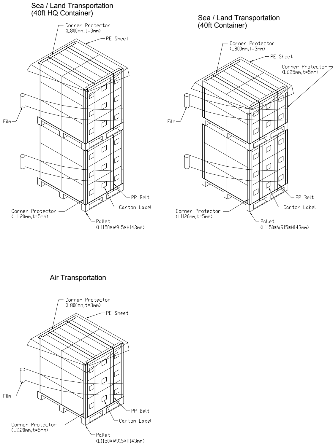
Figure. 7-2 Packing method
