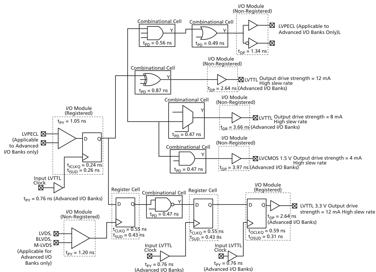
Figure 2-2 • Timing Model
