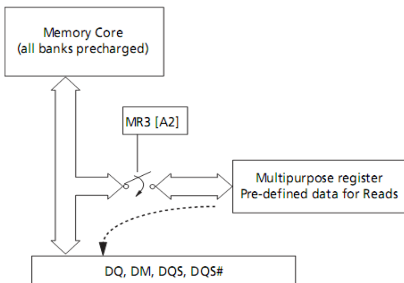
MPR Block Diagram
