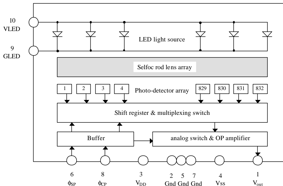
Figure 2 Functional block diagram of M106-A6.
