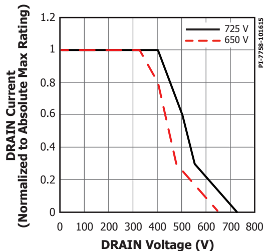
Figure 8. Maximum Allowable Drain Current vs. Drain Voltage.
