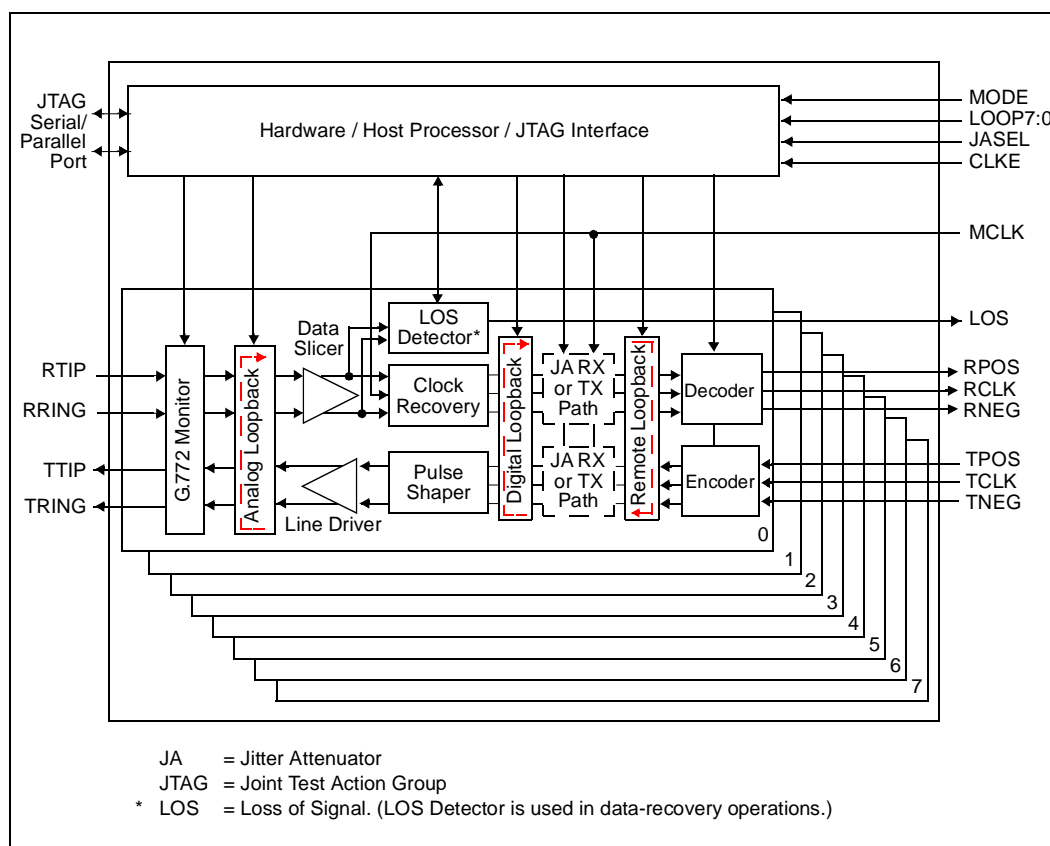
Figure 1. Intel® LXT384 Transceiver High-Level Block Diagram
