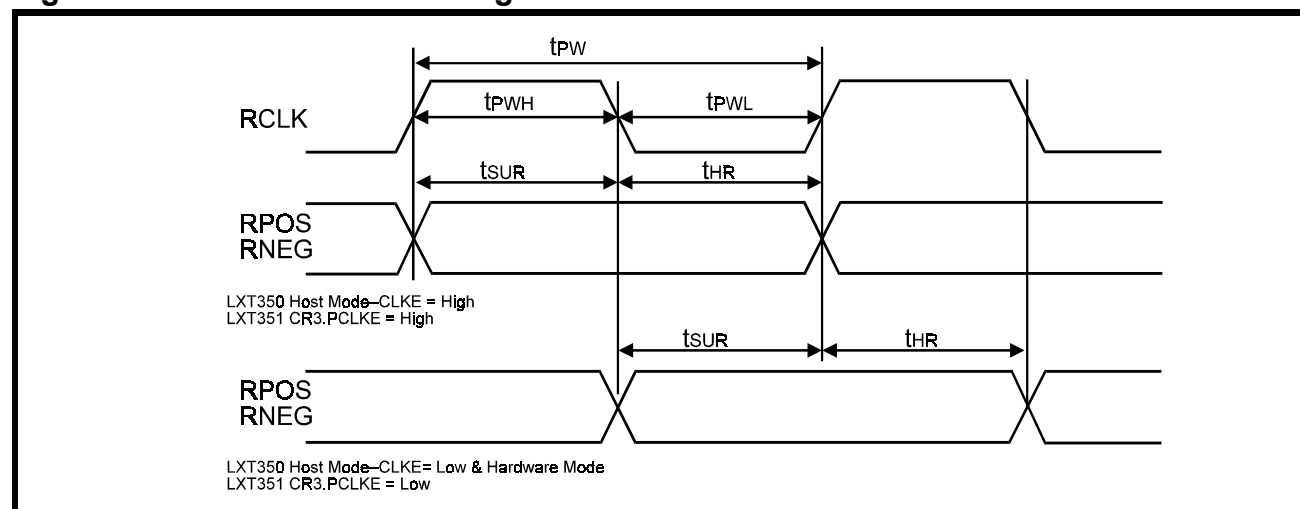
Figure 19: Receive Clock Timing
