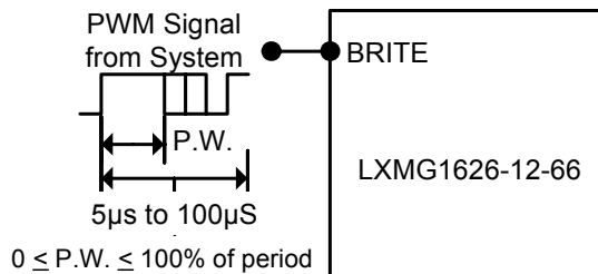
Figure 1A – PWM Brightness Control
