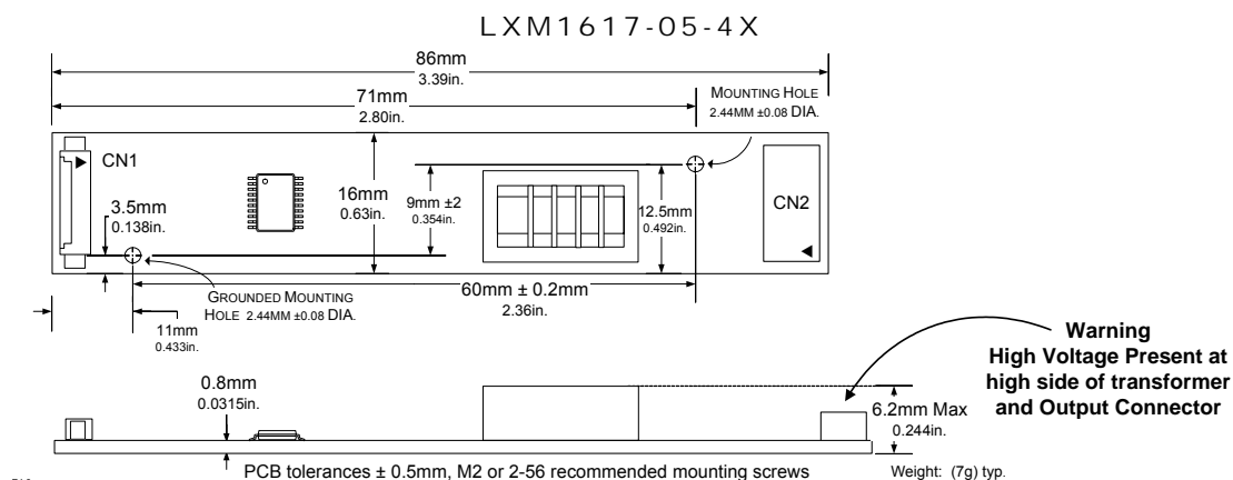
PHYSICAL DIMENSIONS
