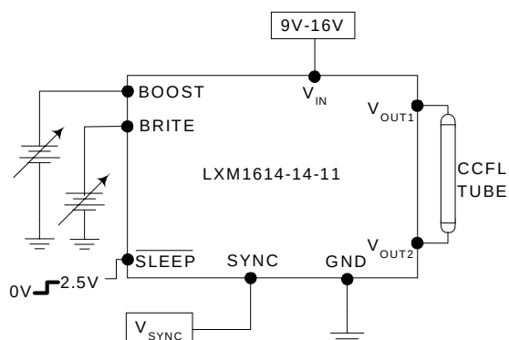
Figure 11 - Brightness Control
