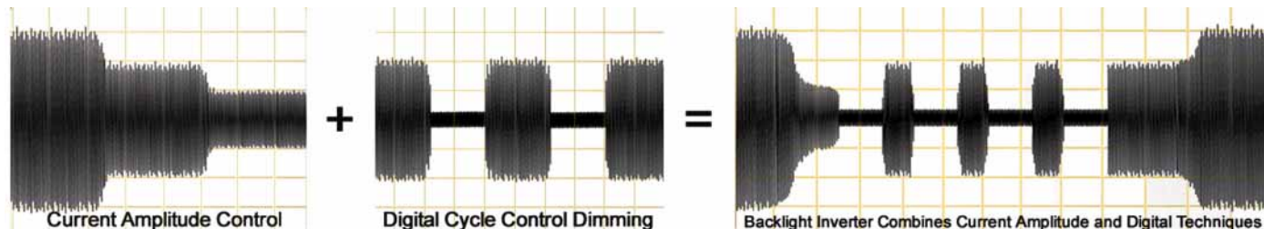
Figure 2 — LXM1614 Combines Current Amplitude and Digital Techniques
