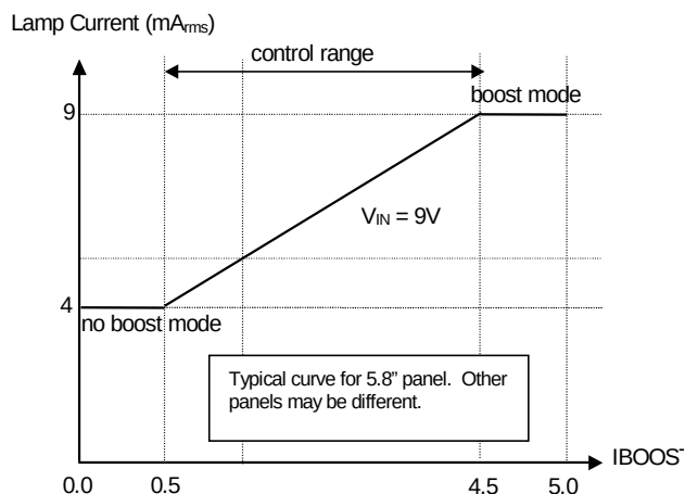
Figure 9 - Maximum lamp current as a function of the Boost control (CN1-6)
