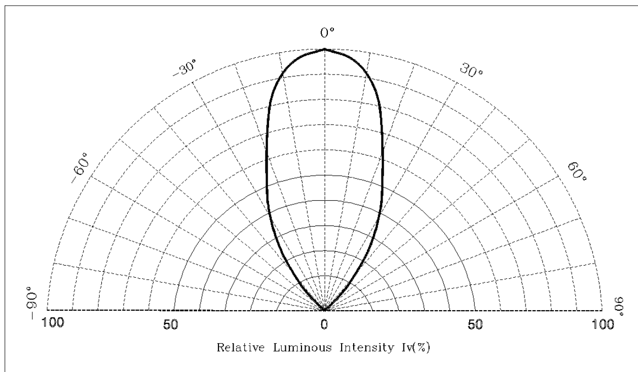
Fig. 4 Radiation Characteristics
