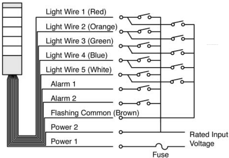
Diagram #2 - Continuous and Flashing with Alarm(s) (24V DC)
