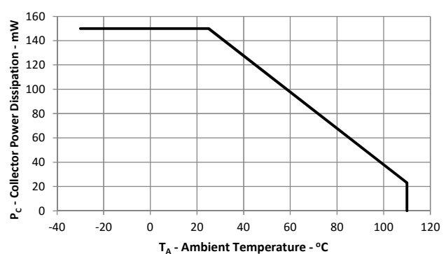
Fig.2 Collector Power Dissipation vs. Ambient Temperature
