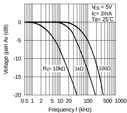
Fig.11 Frequency Response
