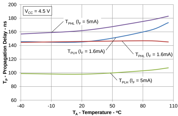
Figure 9: Propagation Delays vs. Temperature
