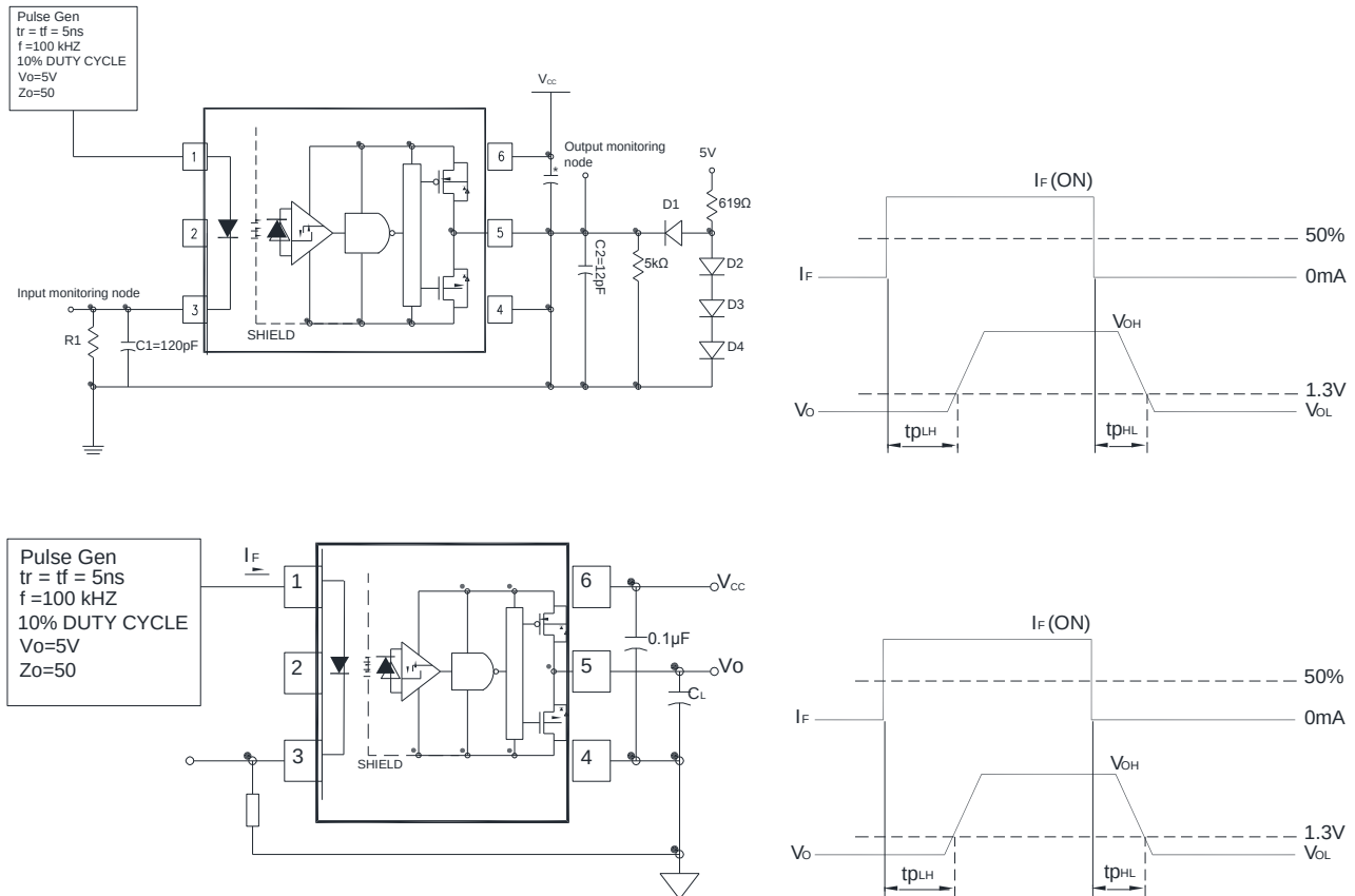
Figure 1 : tr, tf, t PLH and t PHL Test Circuit and Waveforms
