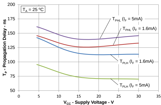
Figure 11: Propagation Delays vs. V_{CC}
