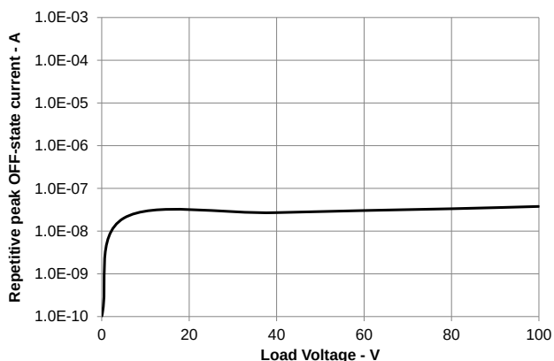
Fig 6. Repetitive peak OFF-state current vs. Load voltage
