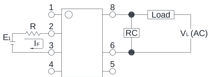
Fig 9. Basic diagrams
