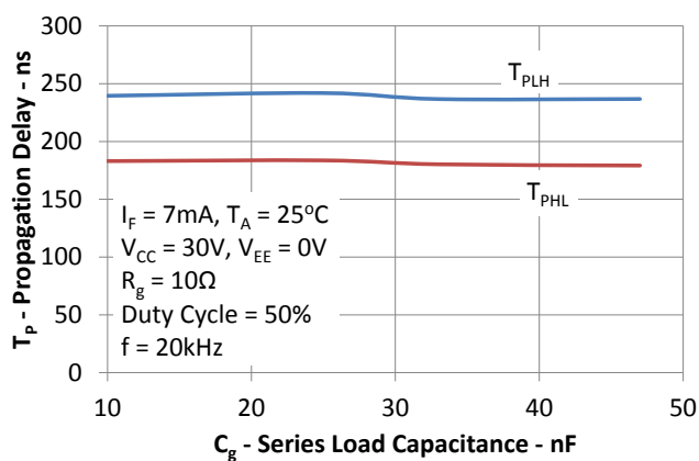
Figure 12: Propagation delays vs. C_g
