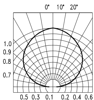
Fig.6 Spatial Distribution
