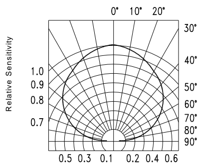
FIG.5 SENSITIVITY DIAGRAM
