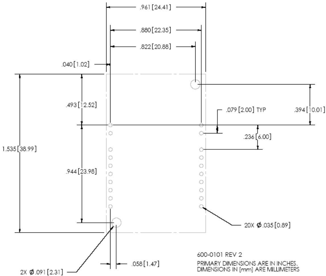
Figure 12 LTP5900 Mote Footprint
