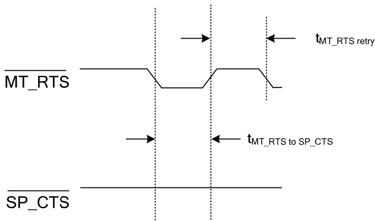
Figure 9 \overline{\text{MT\_RTS}} Timeout Behavior
