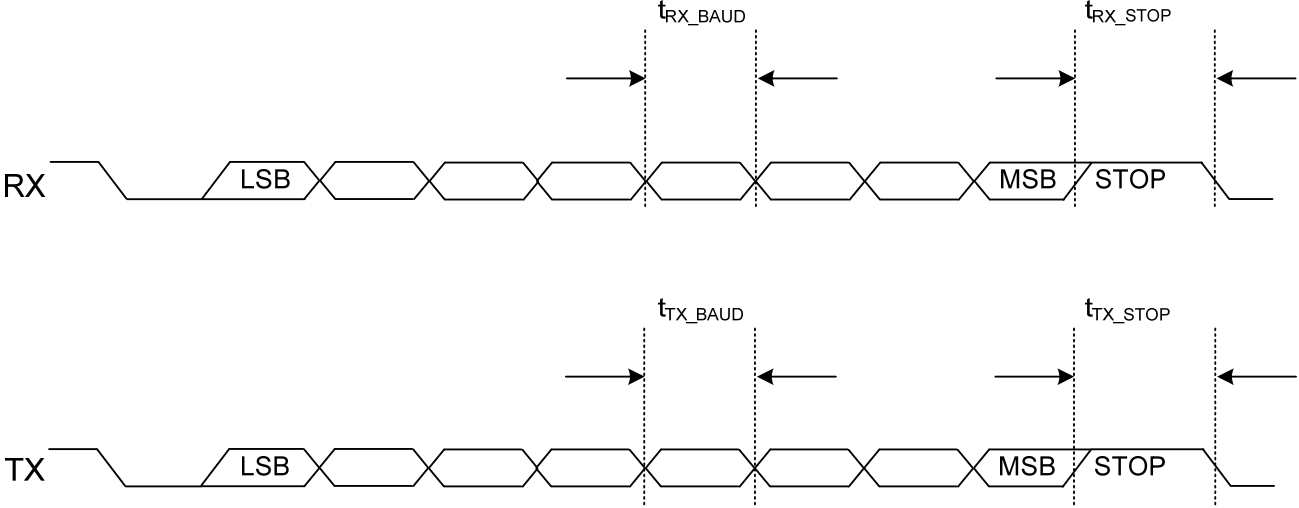
Figure 7 Byte-level Timing
