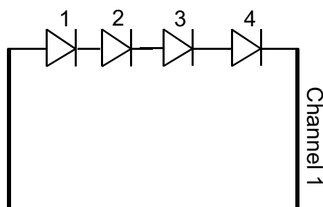
LED Wiring
