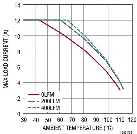
Figure 24. 5V IN to 3.3V OUT Derating Curve, 4-Channel Paralleled, BGA Heat Sink
