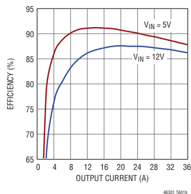
1.2V Output Efficiency, f_{SW} = 500kHz
