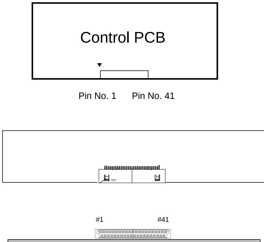
Fig. Connector diagram
