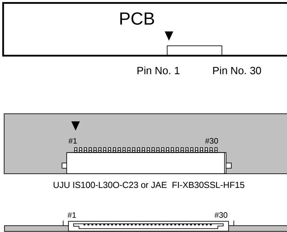
Fig. Connector diagram
