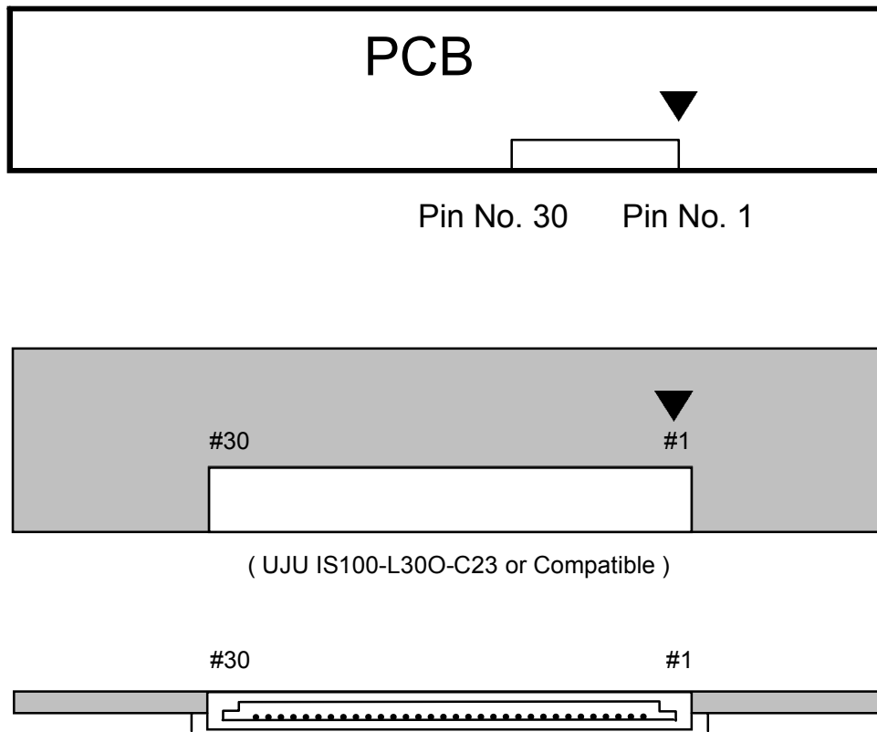
Fig. Connector diagram
