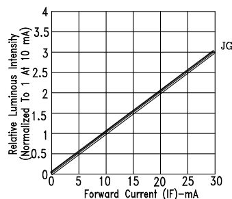
Fig4. RELATIVE LUMINOUS INTENSITY (NORMALIZED TO 1 AT 10 mA) VS. FORWARD CURRENT
