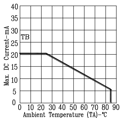
Fig5. MAX. ALLOWABLE DC CURRENT VS. AMBIENT TEMPERATURE.
