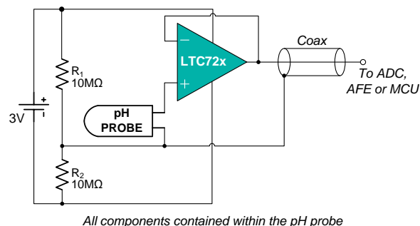
Figure 10. Buffered pH Probe
