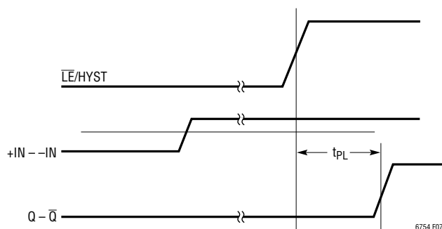
Figure 7e. Latched Output Disabled
