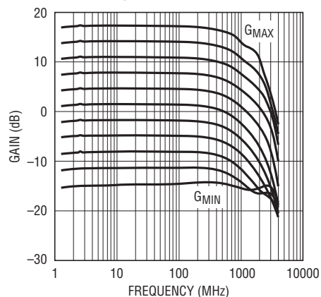
Differential Gain (Sdd21) vs Frequency Over 11 Gain Settings
