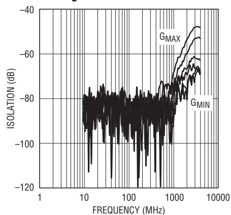
Differential Reverse Isolation (Sdd12) vs Frequency Over 6 Gain Settings
