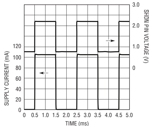
SHDN Supply Current Time Domain Response
