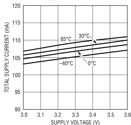
Supply Current vs Supply Voltage Over Temperature
