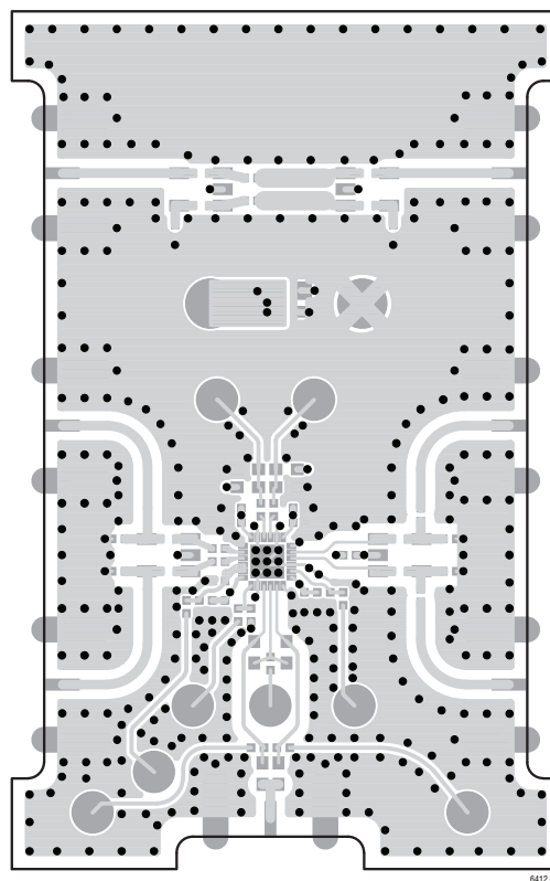
Figure 2. Top Metal for DC1464A. Test Circuit A
