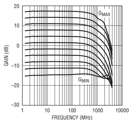
VGA Gain vs Frequency Over Gain Control Range
