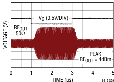
10dB Gain Control Step 70MHz Time Domain Response
