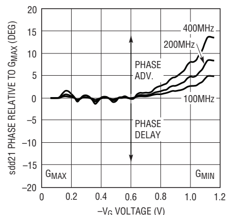
Relative Phase (Sdd21) vs Control Voltage Over Frequency
