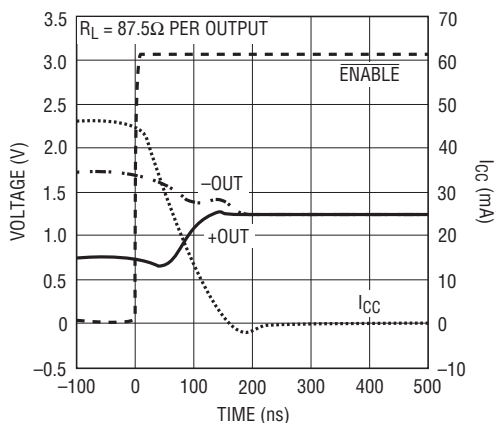
Turn-Off Time
