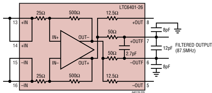
Figure 5. LTC6401-26 Internal Filter Topology Modified for Low Filter Bandwidth (Three External Capacitors)
