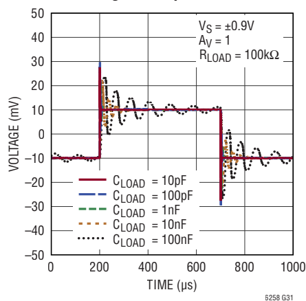
Small-Signal Response
