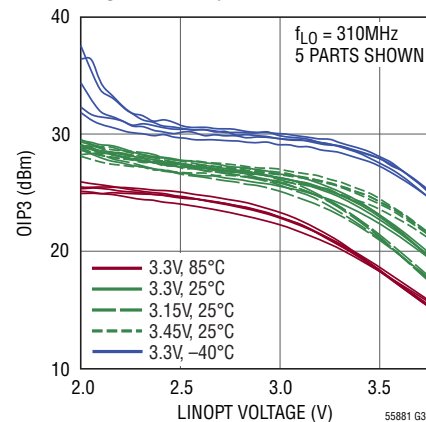
Output IP3 vs LINOPT Voltage ( f_{RF1} = 2140MHz , f_{RF2} = 2141MHz , P_{LOM} = 0dBm )
