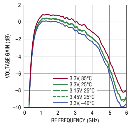
Voltage Gain vs RF Frequency ( P_{LOM} = 0dBm or P_{LOM} = 10dBm )
