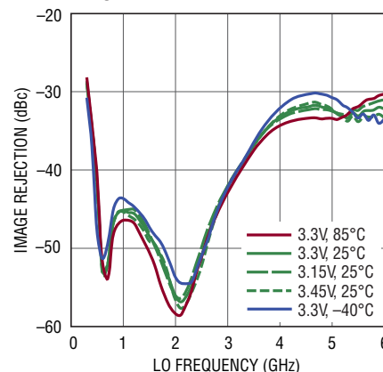
Image Rejection vs LO Frequency ( P_{LOM} = 0dBm )
