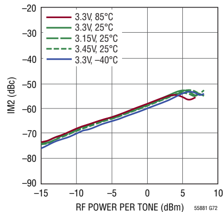
Output IM2 vs RF 2-Tone Power ( P_{LOM} = 0dBm , f_{RF} = 2140MHz , f_{IM2} = 2130MHz )
