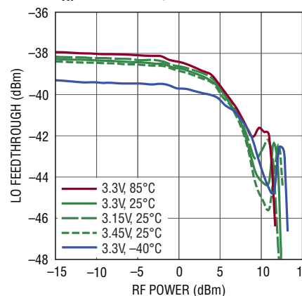
LO Feedthrough to RF Output vs RF Power ( P_{LOM} = 0dBm , f_{RF} = 2140MHz )
