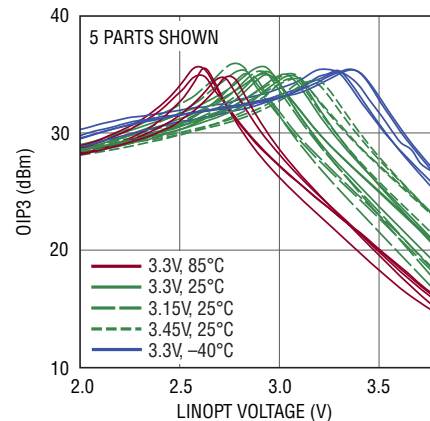
Output IP3 vs LINOPT Voltage ( f_{LO} = 900MHz , P_{LOM} = 0dBm )
