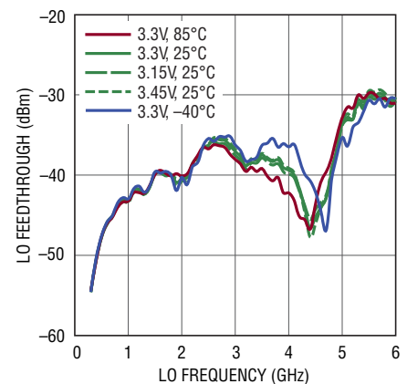
LO Feedthrough to RF Output vs LO Frequency ( P_{LOM} = 0dBm )
