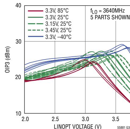
Output IP3 vs LINOPT Voltage ( f_{RF1} = 450MHz , f_{RF2} = 451MHz , P_{LOM} = 0dBm )
