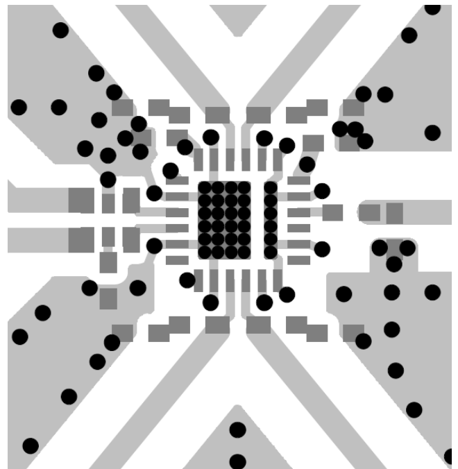
Figure 11. Enlarged View of the Component Side of the Evaluation Board
