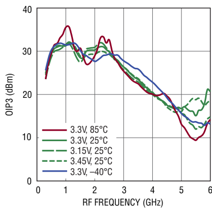
Output IP3 vs RF Frequency ( P_{LOM} = 0dBm )
