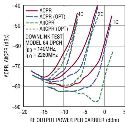
ACPR, AltCPR and ACPR, AltCPR with Optimized LINOPT Voltage vs RF Output Power at 2.14GHz for W-CDMA 1, 2 and 4 Carriers
