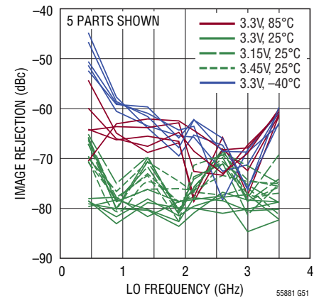
Image Rejection vs LO Frequency After Nulling at 25^\circ C ( P_{LOM} = 0dBm )
