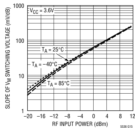
Slope of V_M Comparator Switching Voltage vs RF Input Power at 7000MHz
