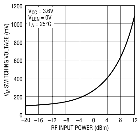
Figure 4. V M Comparator Switching Voltage vs RF Input Power at 12GHz
