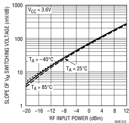
Slope of V_M Comparator Switching Voltage vs RF Input Power at 4000MHz
